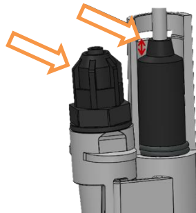
Simplified installation with a single point for measurement and injection
